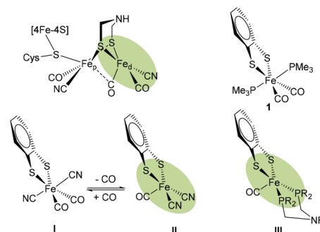
Fig. 1 Schematic structure of the \text{H}_{\text{ox}} state of [FeFe] \text{H}_2 ase active site highlighting the free coordination site in the distal iron ( \text{Fe}_\text{d} ) (top left). Hexa-coordinate (1 and I 4 ) and penta-coordinate (II and III) mononuclear model complexes of \text{Fe}_\text{d} .
