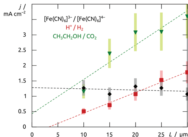
Fig. 8 Steady-state electrochemical current densities j recorded for three distinct reactions at electrodes made out of Pt nanotubes with various lengths L . Experimental conditions: black, 0.05 \text{ M K}_4\text{Fe}(\text{CN})_6 , +0.2 V; red, 0.5 \text{ M H}_2\text{SO}_4 , -0.30 V; green, 0.5 \text{ M H}_2\text{SO}_4 , 0.5 \text{ M ethanol} , +1.1 V (all potentials are reported with respect to Ag/AgCl). The current can vary by up to 20% over time (vertical error bars). The linear fits shown as dashed lines highlight the contrasting behavior of these reactions: the current density increases linearly with the electrode's specific surface area in the case of slow electrochemical transformations (water reduction and ethanol oxidation), whereas it is independent of it for the fast oxidation of hexacyanoferrate(II), which is diffusion-controlled.
