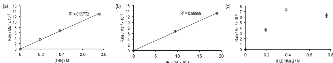
Fig. 2 Initial rate experiments: (a) variation of [TBE]; (b) variation of [ 3 ]; (c) variation of \text{H}_3\text{B}\cdot\text{NMe}_3 . See Table 1 for more details.
