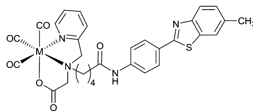
Fig. 16 Structure of ML 20 containing benzothiazole based pendant group conjugated to a tridentate chelate; M = Re I , 99 Tc I or 99m Tc I .
