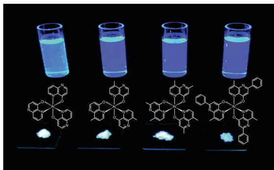
Fig. 5 Emission images of \text{AlND}_3 , \text{AlmND}_3 23 , \text{AlmmND}_3 24 , and \text{AlmpND}_3 25 recorded in solution and solid state under irradiation by UV light. (Reproduced with permission from ref. 16. Copyright 2009, American Chemical Society.)
