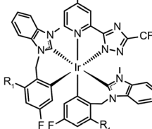
55: R 1 = H, R 2 = t Bu (fbmb) 2 Ir(bptz) 56: R 1 = F, R 2 = H (dfbmb) 2 Ir(fptz)
