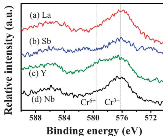
Fig. 7 X-ray photoelectron spectra of Cr 2p of (a) La-Cr, (b) Sb-Cr, (c) Y-Cr, and (d) Nb-Cr codoped \text{SrTiO}_3 . The peaks assigned to \text{Cr}^{3+} and \text{Cr}^{6+} are indicated by dashed and dotted lines, respectively.
