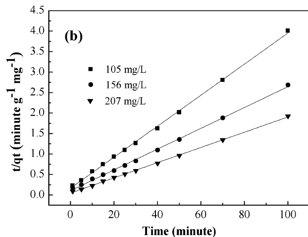
Fig. 7 Pseudo-first-order kinetic model (a), pseudo-second-order kinetic model (b) for adsorption of Cr(vi) onto PAN/PANI nanofiber mat.
