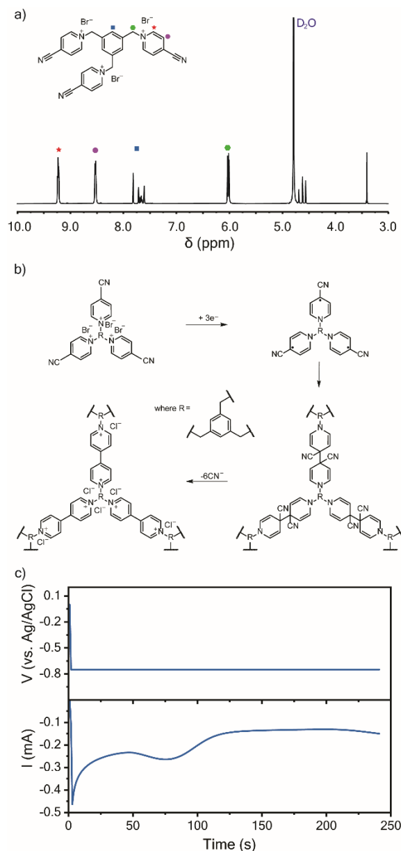
Figure 1. Synthesis and formation of the crosslinked-viologen network. a) 1 H-NMR spectra of TPM bromide salt. b) The electropolymerization mechanism resulting in a crosslinked-viologen network (PTPM). c) The output current during potentiostatic electropolymerization onto a Au/Ti EQCM-D sensor. The electrolyte was 5 mM TPM in aqueous 0.1 M NaCl. The Au/Ti crystal was the working electrode with a Ag/AgCl reference electrode and platinum plate counter electrode.
