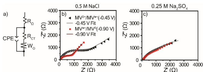
Figure 6. a) The equivalent circuit used to model the EIS data. Nyquist plots for PTPM in b) 0.5 M NaCl and c) 0.25 M \text{Na}_2\text{SO}_4 with their curve fits. EIS was conducted at -0.45 V and -0.90 V vs. Ag/AgCl (sat.) with an amplitude of 10 mV in a frequency range of 5 \times 10^6 Hz to 0.1 Hz (10 steps per decade). Bode plots are found in Figures S5 and S6.
