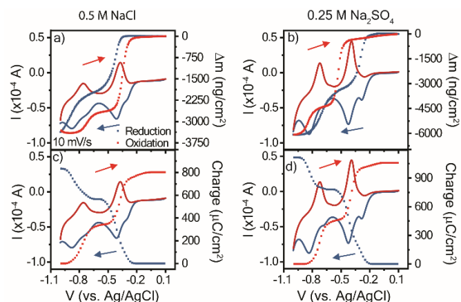
Figure 3. Cyclic voltammograms at 10 mV/s with overlaid mass profiles (a-b) and charge profiles (c-d). The supporting electrolyte was a) and c) 0.5 M NaCl or b) and d) 0.25 M Na 2 SO 4 . Poly(1,3,5-tris(4-cyanopyridinio)mesitylene) (PTPM) on a Au/Ti EQCM-D crystal was the working electrode, and Ag/AgCl reference electrode and platinum plate counter electrode were used. The legend in a) applies to all panels. The cyclic voltammogram is the solid curve, and the charge or mass
