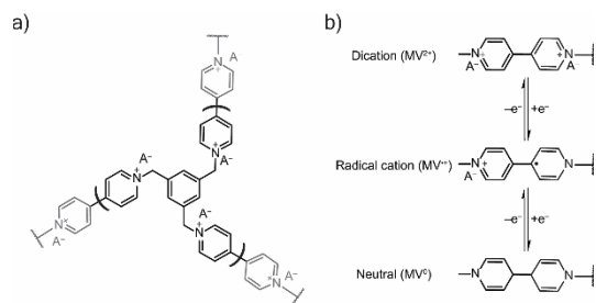
Figure 7. a) the viologen crosslinked network from electropolymerization of TPM salt. b) The redox mechanism of the viologen pendant group with both charge and ion transport, where A^- is an anion.
