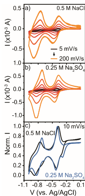
Figure 2. Cyclic voltammograms at varying scan rates for poly(1,3,5-tris(4-cyanopyridinio)mesitylene) (PTPM) in a) 0.5\text{ M NaCl} and b) 0.25\text{ M Na}_2\text{SO}_4 aqueous electrolyte. c) Normalized cyclic voltammograms at 10\text{ mV/s} for both electrolytes. PTPM electropolymerized on the Au/Ti EQCM-D crystal was the working electrode with a Ag/AgCl reference electrode and platinum plate counter electrode. The legend in a) applies to b).
