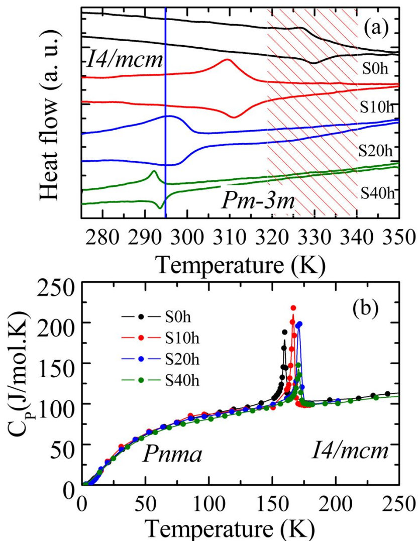
Figure 3 – (a) DSC cycling measurements. The vertical bar indicates the room temperature and the hachured region of the solar cell working temperature range. (b) Molar heat capacity as a function of temperature of pelletized \text{MAPbI}_3 annealed at T_A = 250\text{ }^\circ\text{C} (523 K) for different annealing times.
