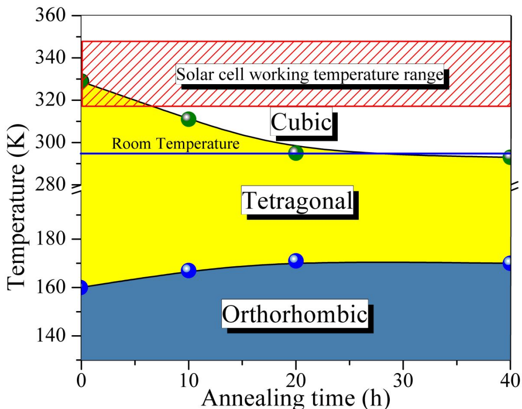
Figure 6 – Phase diagram proposed for the \text{MAPbI}_3 halide perovskite taking into account the observed shift in the phase transition temperature with different annealing conditions. The horizontal bar corresponds to room temperature, and the hatched region indicates the solar cell working temperature range.
