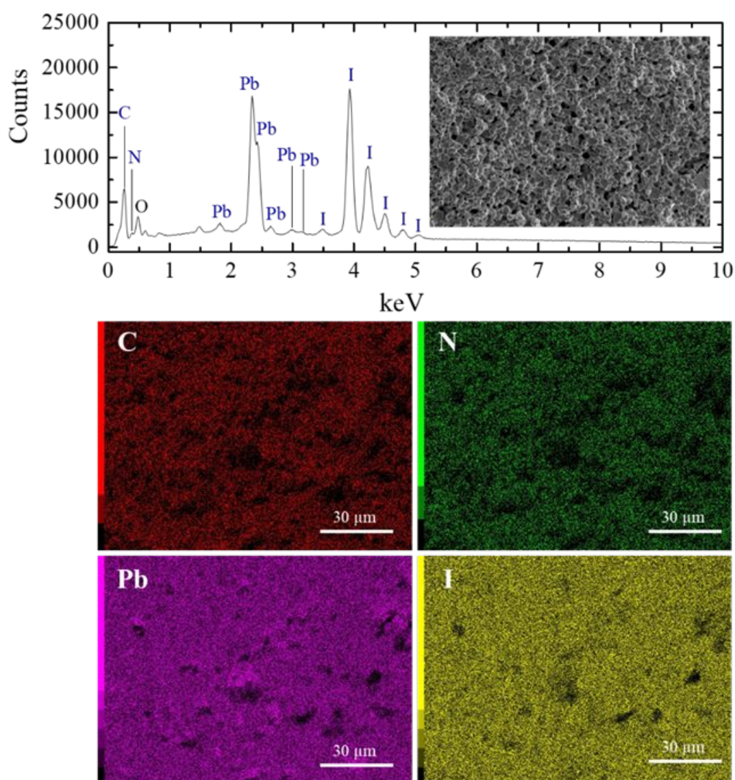
Figure 1 – EDS spectrum and elemental map analysis obtained from a fractured surface of S40h sample.
