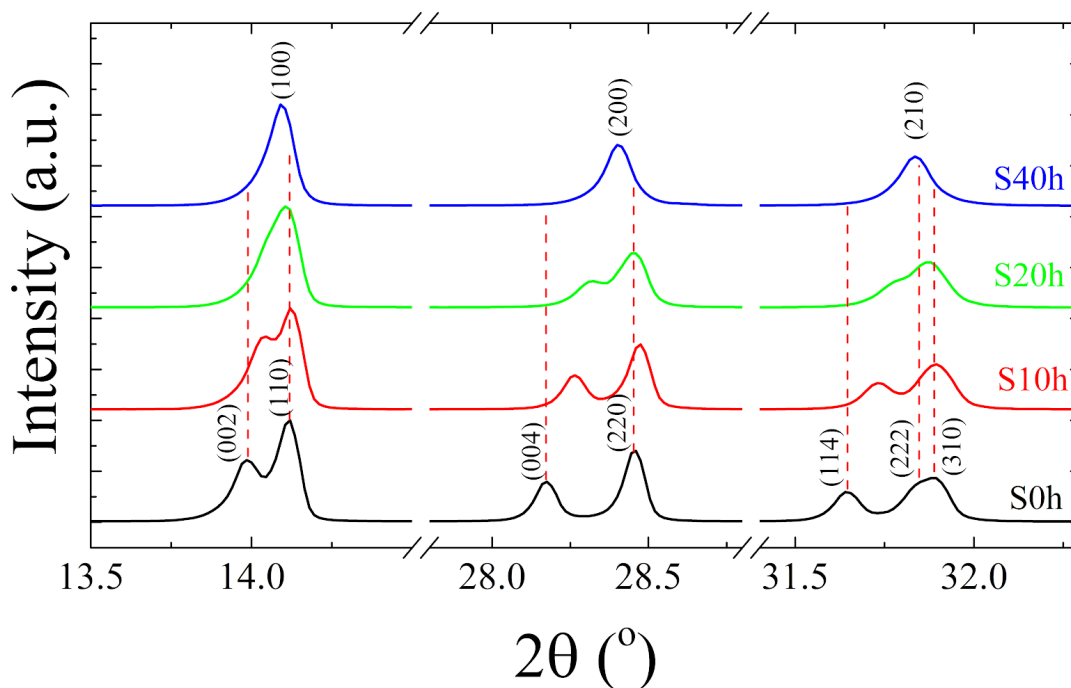
Figure 2 – Room-temperature X-ray diffraction patterns of the pelletized MAPbI 3 sample after being submitted to a heat treatment at T = 250 °C for different annealing times, t = 0, 10, 20, and 40 h.
