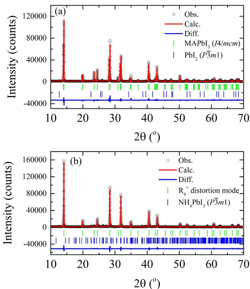
Figure 4 – X-ray powder diffraction data and Rietveld refinements at room temperature of the (a) MAPbI 3 as-compacted sample and (b) submitted to thermal annealing at 250 °C for 40 hours.
