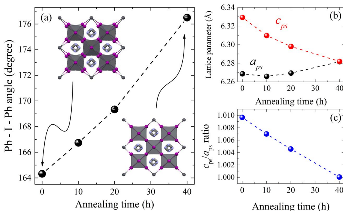
Figure 5 – Structural parameters of the \text{MAPbI}_3 samples submitted to thermal annealing at 250 °C (523 K) and different annealing time. (a) the Pb-I-Pb bond angle changing to almost 180°; insets illustrate rotation of \text{PbI}_6 octahedra along the c -axis. (b) pseudocubic lattice parameters and (c) variation of lattice parameter ratio, c_{ps}/a_{ps} , which reaches 1 for 40h annealing time.
