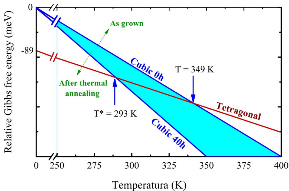
Figure 8 – Schematic of the Gibbs free energy as a function of temperature. At T = 0 K, the energies correspond to the internal energy of each system and were computed within the DFT approach and used the cubic system as a reference. As the temperature increases, the configuration entropy is responsible for different phase transition temperatures from tetragonal to cubic, indicated by 293 and 349 K. The configurational entropy is larger for the sample that was annealed for 40h.
