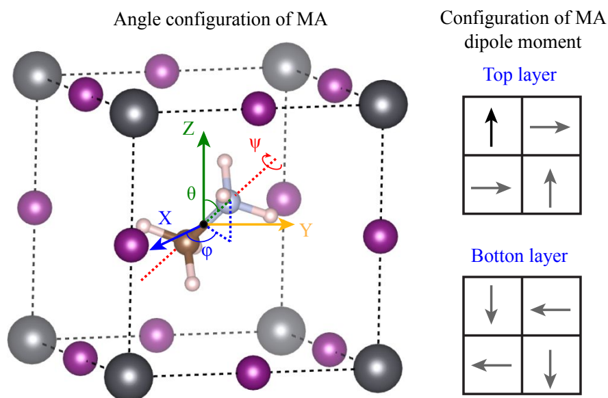
Figure 7 – The left panel indicates the rotational angle configuration of the MA molecule (N, C and H are represented by blue, brown, and pink spheres, respectively) in one cage of Pb (gray spheres) and I (purple spheres). \theta and \phi represent the angles with respect to the X and Z direction, while \psi is the rotation around the axis that pass through the C-N bond. The geometric center of MA molecule was considered as the rotation point, which does not change for any rotation operation. The right panel indicates the initial (non-relaxed) configuration for the most stable dipole orientation for the MA molecule. The black arrow showed the system allowed to relax, while the gray arrows were considered fixed.
