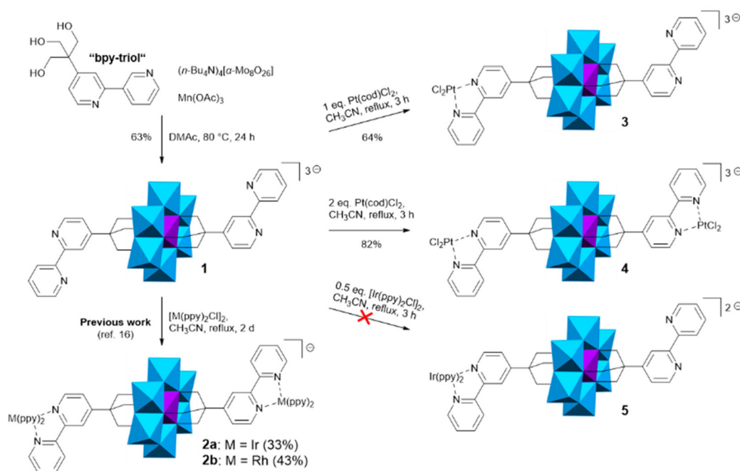
Fig. 1 Schematic representation of the synthesis of the symmetric and asymmetric complexes of \text{bpy} \cdot [\text{MnMo}_6\text{O}_{24}] \cdot \text{bpy} (1) with \text{PtCl}_2 fragments. The respective tetra( n -butyl)ammonium (TBA) counterions are omitted for clarity. Colour scheme for the POM moiety: Mo: blue, Mn: purple.
