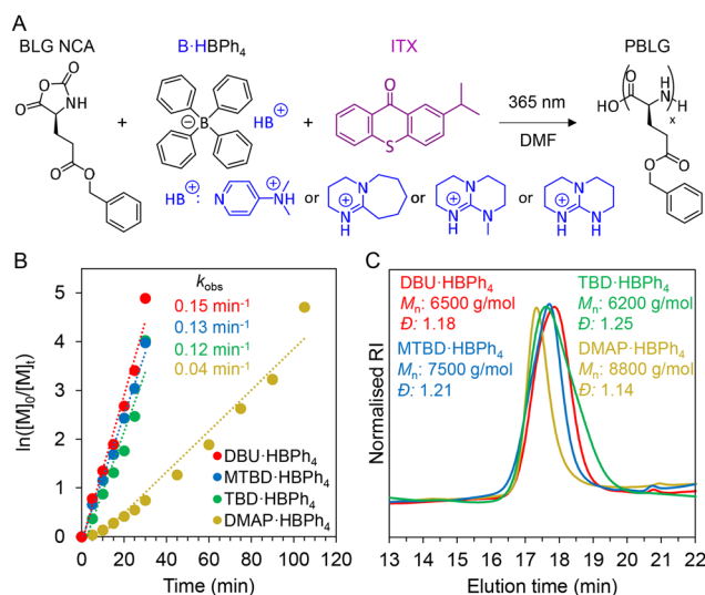
Fig. 2 Schematic of synthetic route for polypeptides using different PBGs, (B) kinetic plot of \ln([M]_0/[M]_t) versus time for BLG NCA photo-ROP with different PBGs ( [M] = 0.4 M, [M]_0/[I]_0 = 50 ) in DMF, and (C) normalized SEC traces of corresponding polypeptides.
