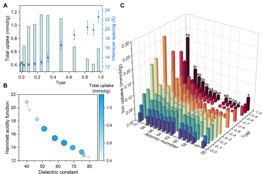
Fig. 2 Ion uptake behavior of 2D channels in DMF–water media. (A) Total ion uptake (mmol/g) and corresponding interlayer spacing as a function of DMF fraction x_{\text{DMF}} (from left to right, DMF–water molar ratios are 0, 1 : 30, 1 : 10, 1 : 5, 1 : 3, 1 : 2, 1 : 1, 2 : 1, 5 : 1, 10 : 1, and 35 : 1). (B) Bubble plot showing the three-dimensional correlation of dielectric constant, Hammett acidity function and total uptake. Dielectric constant and acidity function values for DMF–water mixtures are taken from literature and summarized in Table S1. (C) Ion uptake of individual REE ion versus DMF–water ratio, showing preferential uptake for heavy elements with higher DMF fraction.
