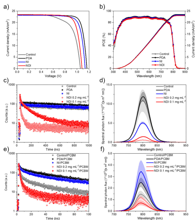
Fig. 4 Optoelectronic characteristics of NI/NDI-based perovskite solar cells. (a) J - V curves of the devices with different passivation layers in comparison to the control device without any treatment, with a scan rate of 10 \text{ mV s}^{-1} . (b) IPCE spectra and calculated photocurrent integrated over the standard AM 1.5G solar spectrum. In agreement to the J - V data no change in the spectra is observed. (c) and (e) Time-resolved photoluminescence spectroscopy (TRPL) of perovskite (gray) and modulated films with PDA (black), NI (blue), NDI high concentration (pink) and NDI low concentration (red) on microscope slides without (c) and with (e) the electron-transport material (PCBM). (d) and (f) Steady-state absolute intensity photoluminescence (AIPL) spectra of perovskite (gray) and treated films with PDA (black), NI (blue), NDI (high concentration, pink, and low concentration, red) on FTO/MeO-2PACz without (d) and with (f) the electron-transport layer (PCBM). Error band represents the standard deviation of 5 samples per condition.
