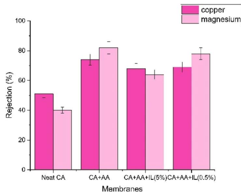
(b) Rejection performance of the membranes at a pressure of 2 bar at pH 7
