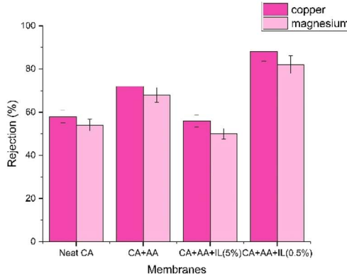
(d) Rejection performance of the membranes at a pressure of 4 bar at pH 7
