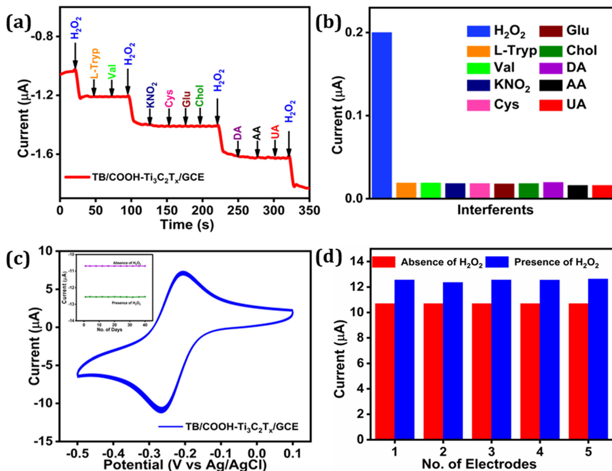
Fig. 6 (a) Effect of interference in H 2 O 2 determination (5 μM) in the presence of other interferents (0.5 mM) in N 2 -saturated 0.1 M PBS (pH 7) and (b) the corresponding bar diagram. (c) CV curve of the TB/COOH-Ti 3 C 2 T x /GCE for 50 continuous cycles. Inset: the plot of day-to-day current response of the fabricated sensor in the presence (green) and absence (pink) of 50 μM H 2 O 2 . (d) Bar diagram comparing the current response with and without H 2 O 2 (50 μM) for five identically fabricated sensors.
