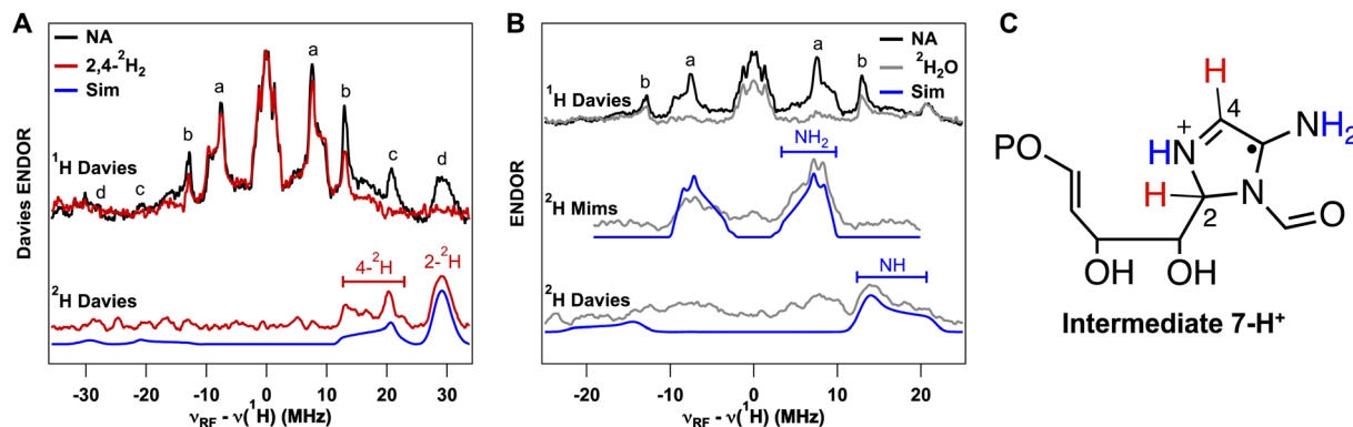
Fig. 3 (A) 1 H and 2 H Davies ENDOR spectra for the AtThiC reaction quenched after 6 minutes using NA AIR or 2,4- 2 H 2 AIR. The 2 H Davies ENDOR spectrum for the 2,4- 2 H 2 AIR sample was scaled to the frequency of 1 H for easier comparison. (B) 1 H Davies and frequency-scaled 2 H Davies and Mims ENDOR spectra comparing the NA AIR samples made in H 2 O or 2 H 2 O. Experimental data are shown in black or grey. Spectral simulations are shown in blue. (C) The structure of proposed intermediate 7-H + with positions contributing to the observed HFI labeled in red and blue. Conditions: frequency = 34 GHz, temperature = 15 K. 1 H and 2 H Davies: \pi/2 = 12 ns, inversion pulse = 80 ns, \tau = 300 ns. 2 H Mims: \tau = 260 ns. Simulations: (A) A(2\text{-}^2\text{H}) = [8.4, 9.0, 9.6] MHz, A(4\text{-}^2\text{H}) = [3.7, 6.3, 7.4] MHz. (B) Mims: A_1^2\text{H} = [2.6, 0.7, 3.2] MHz, A_2^2\text{H} = [2.2, 3.1, 1.0] MHz. Davies: A^2\text{H} = [4.4, 6.8, 3.8] MHz.
