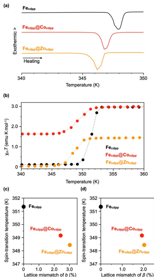
Fig. 4 (a) DSC profiles of \text{Fe}_{\text{cdpp}} (black), \text{Fe}_{\text{cdpp}}@\text{Co}_{\text{cdpp}} (red) and \text{Fe}_{\text{cdpp}}@\text{Zn}_{\text{cdpp}} (orange) upon heating at a rate of 1 \text{ K min}^{-1} . (b) Temperature-dependent magnetic susceptibility of \text{Fe}_{\text{cdpp}} (black), \text{Fe}_{\text{cdpp}}@\text{Co}_{\text{cdpp}} (red) and \text{Fe}_{\text{cdpp}}@\text{Zn}_{\text{cdpp}} (orange) upon heating at a rate of 1 \text{ K min}^{-1} under a magnetic field of 1 \text{ T} (see Fig. S13 for the cooling process, SI). The \chi_{\text{m}}T values were calculated assuming a 50 : 50 molar ratio between \text{Fe}_{\text{cdpp}} and \text{M}_{\text{cdpp}} ( \text{M} = \text{Co}, \text{Zn} ) in the core-shell crystals. Plots of spin-transition temperatures ( T_{1/2} ) versus core/shell lattice constant mismatch at (c) b and (d) \beta .
