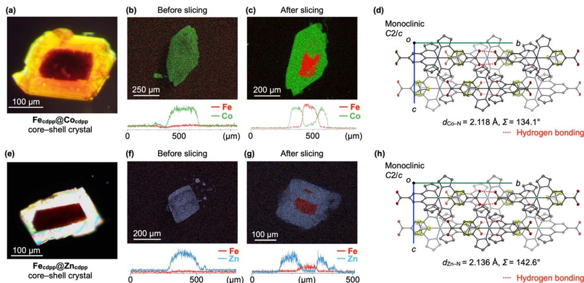
Fig. 3 (a) POM image of \text{FeCdpp@CoCdpp} . (b and c) SEM-EDX elemental maps (top) and total area traces (bottom) of \text{FeCdpp@CoCdpp} (b) before and (c) after slicing by a ultramicrotome. (d) Crystal structure of \text{CoCdpp} in the outer shell along the a -axis. (e) POM image of \text{FeCdpp@ZnCdpp} . (f and g) SEM-EDX elemental maps (top) and total area traces (bottom) of \text{FeCdpp@ZnCdpp} (f) before and (g) after slicing by a ultramicrotome. (h) Crystal structure of \text{ZnCdpp} in the outer shell along the a -axis.
