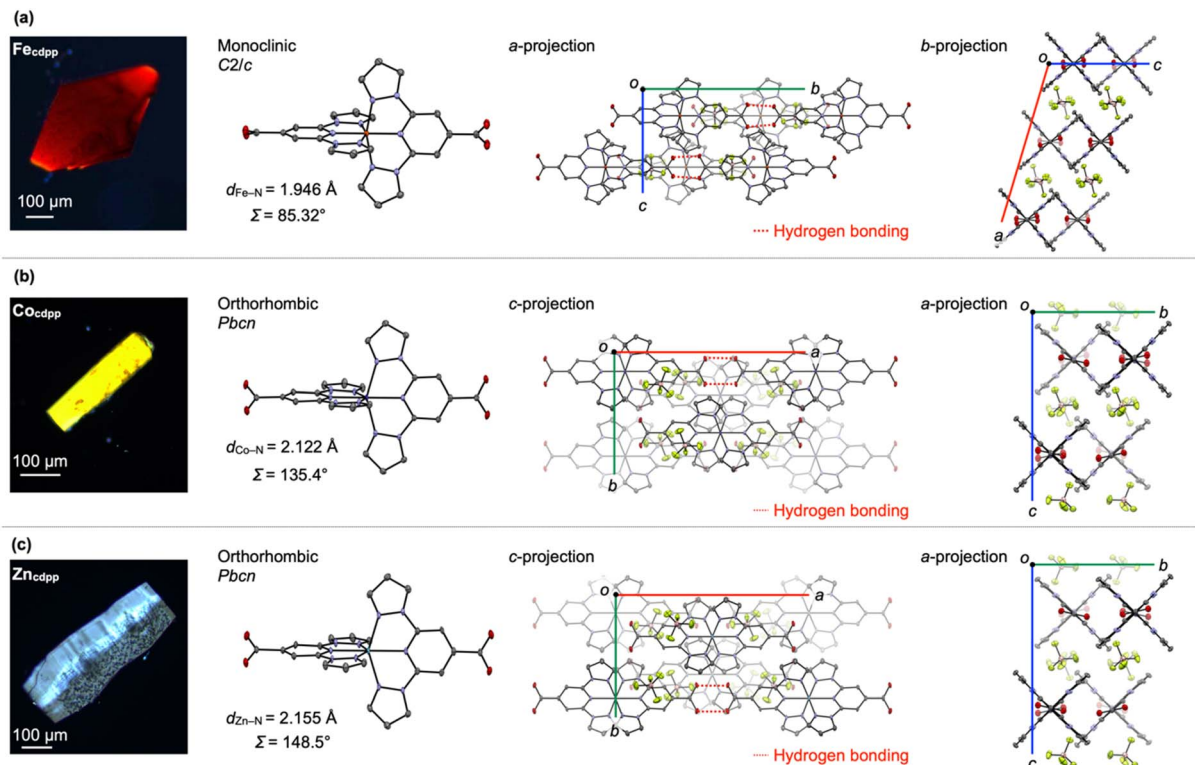
Fig. 2 POM images and X-ray crystal structures (molecular and packing structures) of (a) \text{FeCdpp} , (b) \text{CoCdpp} and (c) \text{ZnCdpp} . Color code: carbon = gray, nitrogen = blue, oxygen = red, iron = orange, cobalt = purple, zinc = sky blue, fluorine = green, boron = pink. Hydrogen atoms have been omitted for clarity.
