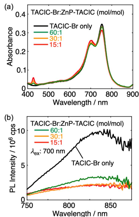
Fig. 6 (a) UV-vis-NIR absorption spectra and (b) fluorescence spectra of TACIC-Br/ZnP-TACIC in a mixture of \text{CHCl}_3 and MeOH (1 \times 10 -5 M, 50 : 50, v/v). The inset depicts the molar ratio of TACIC-Br : ZnP-TACIC.
