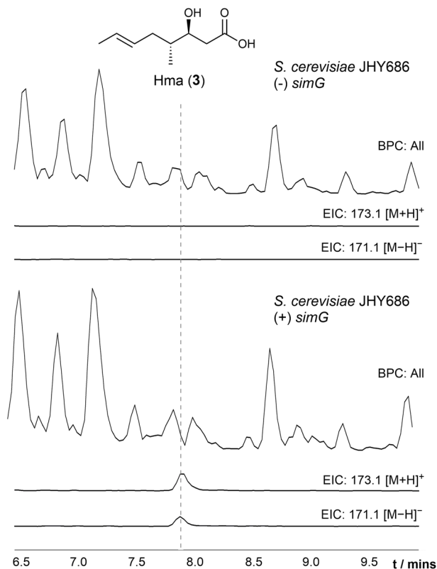
Fig. 2 Detection of 3 R -hydroxy-4 R -methyl-6 E -octenoic acid (Hma) from S. cerevisiae JHY686. LC-ESI-MS analysis of ethyl acetate extracts from culture medium of S. cerevisiae JHY686 in the absence (top) and presence of the simG gene (bottom). In each case, the base peak chromatograms and extracted ion chromatograms for [M + H]^+ , m/z = 173.1 and [M - H]^- , m/z = 171.1 corresponding to Hma (3), are shown. Production of 3 is only observed when expressing the simG gene. Purification followed by NMR spectroscopy verified the structure of the product (ESI Table S2†).
