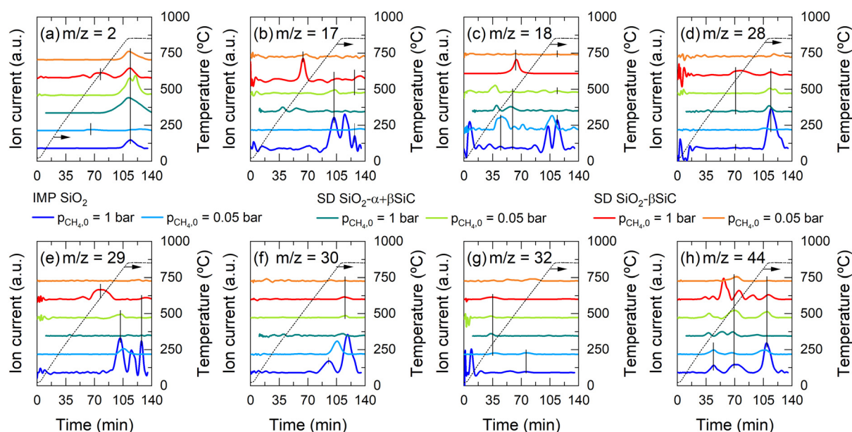
Fig. 4 Evolution of temperature and MS signals over time for each catalyst at different CH 4 partial pressures in the carrier gas. Conditions: P = 1 bar, T 1 = 25 °C, T F = 850 °C, β = 7.5 min -1 , t ox = 30 min, F T = 100 NmL min -1 , W = 50 mg c . O 2 chemisorption occurred for 6 h at 25 °C and 50 NmL min -1 (10% O 2 ).
