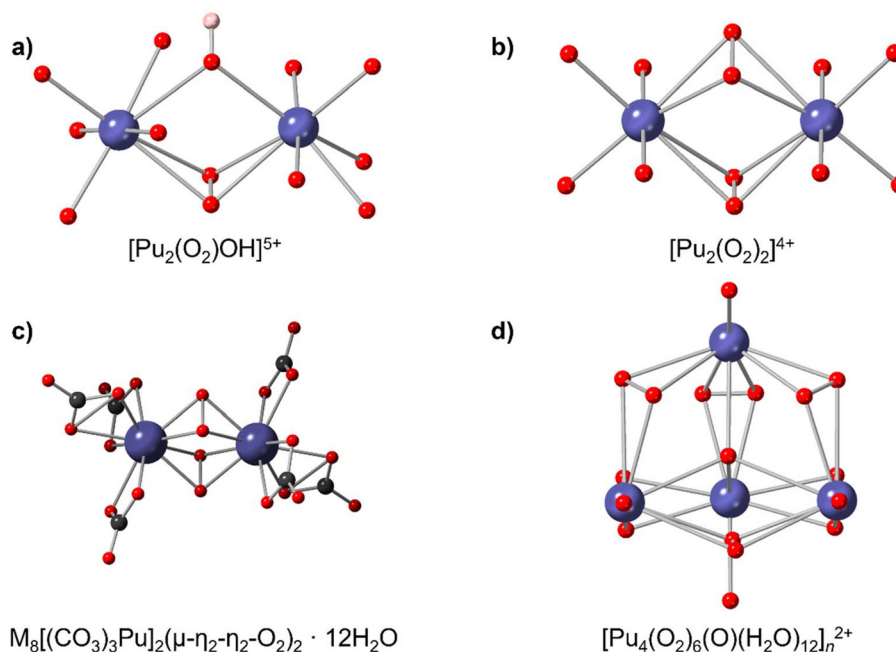
Fig. 9 \text{Pu(IV)} peroxy-complexes such as (a) [\text{Pu}_2(\text{O}_2)(\text{OH})]^{5+} , (b) [\text{Pu}_2(\text{O}_2)_2]^{4+} , (c) \text{M}_8[(\text{CO}_3)_3\text{Pu}]_2(\mu\text{-}\eta_2\text{-}\eta_2\text{-O}_2)_2\cdot 12\text{H}_2\text{O} (where \text{M} = \text{K} or \text{Na} ), and (d) [\text{Pu}_4(\text{O}_2)_6(\text{O})(\text{H}_2\text{O})_{12}]_n^{2+} . Pu, O, C, and H are represented as purple, red, grey, and pink spheres, respectively. Hydrogens on aqua ligands, outer sphere water molecules, and counter cations were omitted for clarity. 95–97
