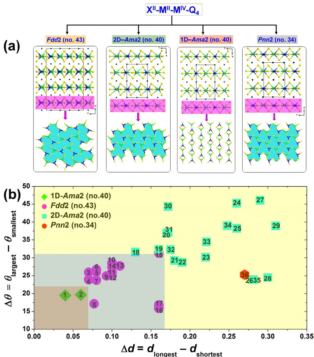
Fig. 3 (a) Comparison of four distinct structural types within the \text{X}^{\text{II}}\text{--M}^{\text{II}}\text{--M}^{\text{IV}}\text{--Q}_4 ( \text{X}^{\text{II}} = Eu, Sr and Ba; \text{M}^{\text{II}} = Zn, Cd, and Hg; \text{M}^{\text{IV}} = Si, Ge and Sn; Q = S, Se) family; (b) the relationship between the degree of structural distortion, quantified by \Delta d ( \Delta d = (d_{\text{longest}} - d_{\text{shortest}}) ) and \Delta\theta ( \Delta\theta = (\theta_{\text{largest}} - \theta_{\text{smallest}}) ) and (\Delta\theta_1 + \Delta\theta_2)/2 , and the space groups. The compounds corresponding to the numbers in this figure are listed in Table S4.†
