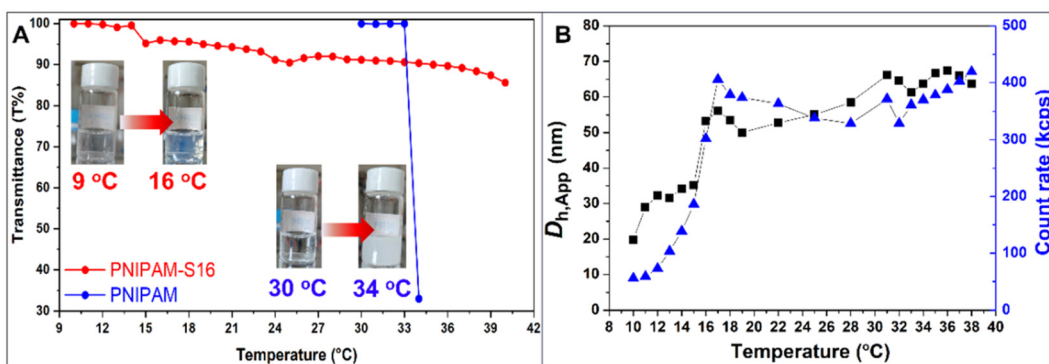
Fig. 3 (A) Transmittance of aqueous solutions of PNIPAM and PNIPAM-S16 (1.0 mg mL -1 , \lambda = 500 nm). (B) Dependence of D_{h,app} and count rate of the aqueous solution of PNIPAM-S16 (1.0 mg mL -1 ) on temperature.
