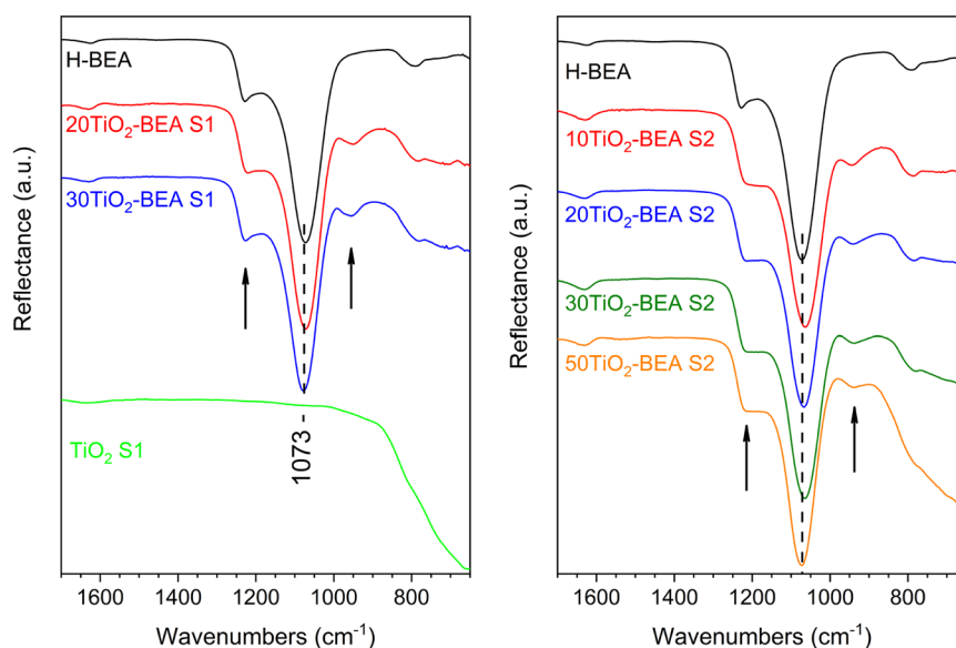
Fig. 6 FTIR spectra of the different composite materials (ATR mode): (left), S1 series, and (right) S2 series (the arrows in both figures depict the bands at about 1230 and 950 \text{cm}^{-1} ).
