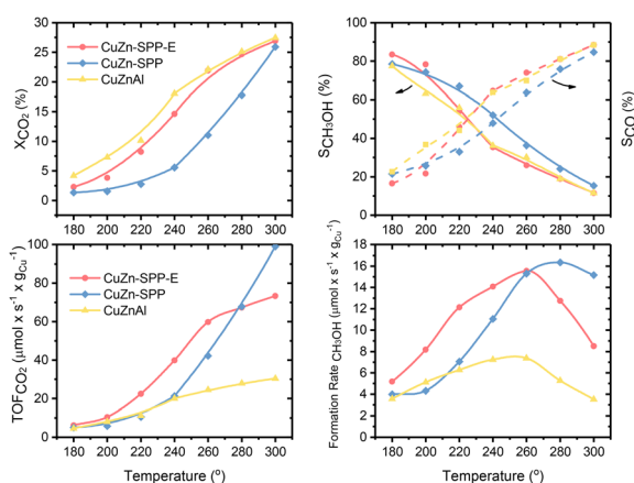
Fig. 2 Catalytic performances of CuZn-SPP-E, compared with CuZn-SPP and Cu/ZnO/Al 2 O 3 : CO 2 conversion, X CO 2 ; selectivity for CH 3 OH, S CH 3 OH and for CO, S CO ; turn-over-frequency of CO 2 per unit Cu, TOF CO 2 ; and the formation rate of CH 3 OH per unit Cu. The test conditions were feeding CO 2 /H 2 = 1/3 at P = 3 MPa and WHSV CO 2 = 9.3 g h -1 g cat -1 .
