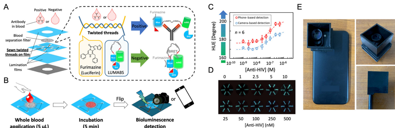
Fig. 41 Thread-based BRET detection of target antibodies to avoid user steps after the addition of sample. (A) Design of the threaded paper stack, with luciferase and its substrate dried on separate threads. (B) Assay workflow. (C) Plot of smartphone-measured luminescence hue versus analyte concentration. (D) Smartphone-acquired BL images for different concentrations of the anti-HIV antibody analyte. (E) Photographs of the smartphone-based imaging device. Figure adapted with permission from ref. 541 Copyright 2020 American Chemical Society.
