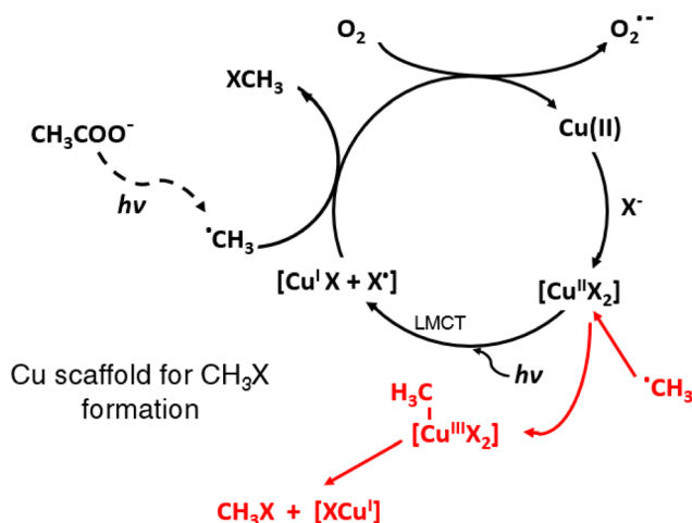
Fig. 1 TM-assisted PVG of halogens using added Cu(II) as an example of aquo-metal halide complex formation followed by (i) ·CH 3 capture of halide atom (X · ) formed by a LMCT process or (ii, shown in red) oxidative addition of ·CH 3 to CuX 2 complex followed by reductive elimination of CH 3 X and subsequent catalytic re-oxidation of Cu(I) by dissolved oxygen or other oxidants in the system.
