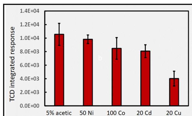
Fig. 15 Impact of added TMs (concentrations given as \mu g mL^{-1} ) on response (generation) of H_2 from photolysis of 5% (v/v) acetic acid at 2 mL min^{-1} (IT = 32 s; repeatability SD: n = 3 ). Uncorrected HS [ H_2 ] in 5% acetic acid is 270 \pm 40 ppm. Ordinate displays integrated response characterizing chromatographic peaks.
