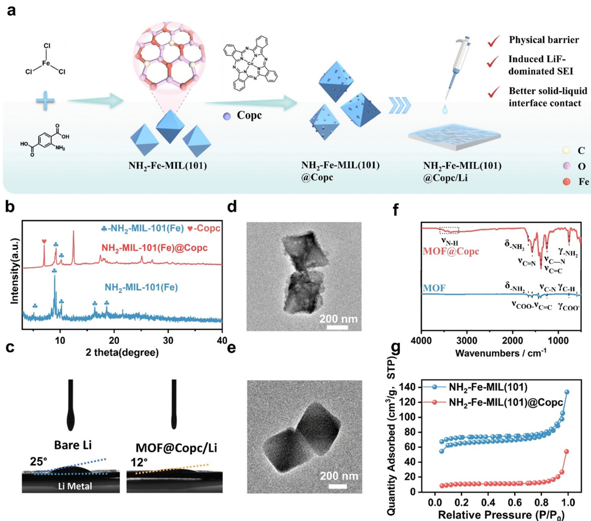
Fig. 3 Characterization of the composite NH 2 -MIL-101(Fe)@Copc (a) schematic diagram of the preparation of NH 2 -MIL-101(Fe) and NH 2 -MIL-101(Fe)@Copc nanocomposite. (b) XRD of NH 2 -MIL-101(Fe) and NH 2 -MIL-101(Fe)@Copc. (c) Contact angle measurement of bare Li and MOF@Copc/Li surfaces. (d) and (e) TEM image of NH 2 -MIL-101(Fe) and NH 2 -MIL-101(Fe)@Copc. (f) FTIR spectra of NH 2 -MIL-101(Fe)@Copc. (g) N 2 adsorption-desorption isotherm.
