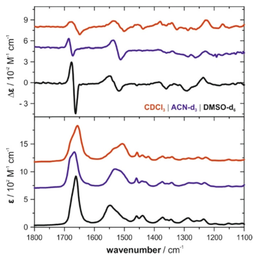
Fig. 1 Comparison of the experimental and computed VCD and IR spectra of (S)- Ace-Trp-N(n-Pr) in \text{CDCl}_3 (0.105 M, 100 \mu\text{m} ), \text{ACN-d}_3 (0.077 M, 200 \mu\text{m} ), and \text{DMSO-d}_6 (0.208 M, 50 \mu\text{m} ).
