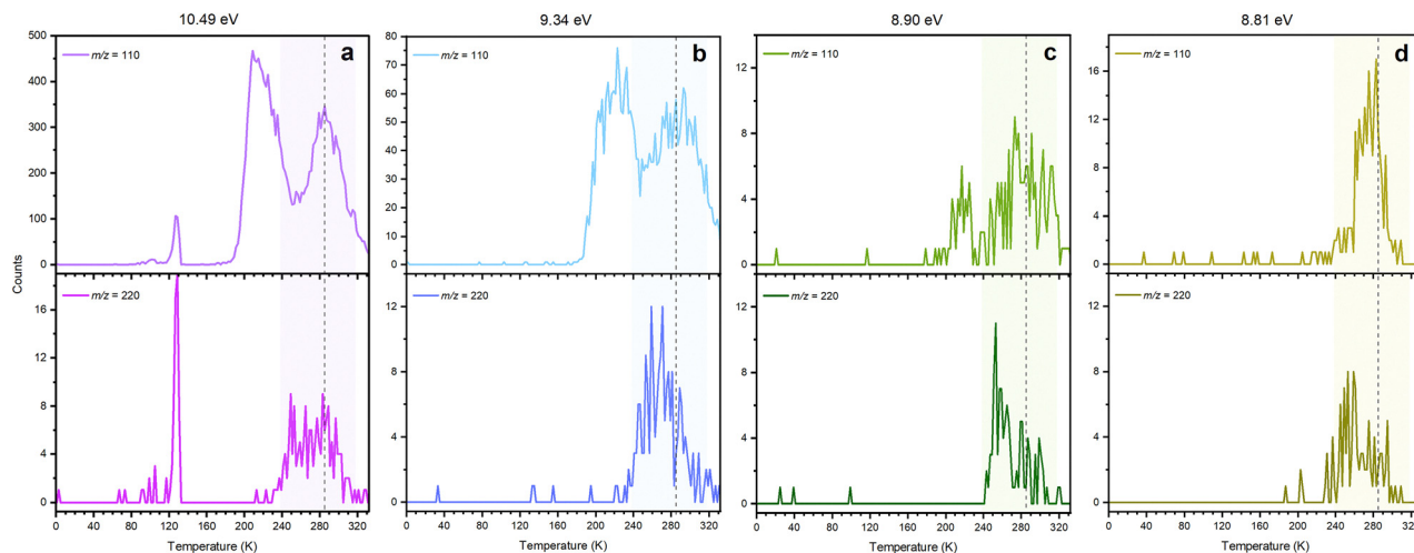
Fig. 9 Compared TPD profiles of m/z = 110 and m/z = 220 from the irradiated \text{H}_2\text{S-CS}_2 ice recorded at 10.49 (a), 9.34 (b), 8.90 (c), and 8.81 eV (d). The dashed line indicates the sublimation peak at 285 K (Peak III).
