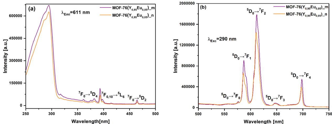
Fig. 12 Excitation ( \lambda_{\text{Emi}} = 611 nm) (a) and emission spectra ( \lambda_{\text{Exc}} = 290 nm) (b) of microcrystalline MOF-76( \text{Y}_{0.95}\text{Eu}_{0.05} ) m compound and nanocrystalline MOF-76( \text{Y}_{0.95}\text{Eu}_{0.05} ) n material.
