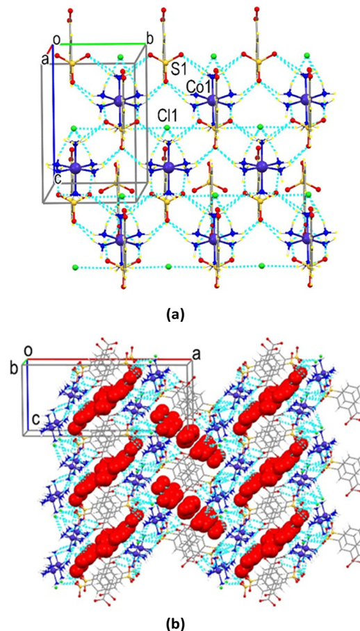
Fig. 3 (a) A fragment of the supramolecular layer in which the [\text{Co}(\text{NH}_3)_6]^{3+} cations are linked by H-bonds with the \text{Cl}^- anions and oxygen atoms of the sulfonate groups in 3 . (b) Formation of channels in the crystal due to bridging of layers by \text{N-H}\cdots\text{O} bonds of sulfonate and carboxylate groups of 3-sb . The solvent water molecules are shown in a space-filling mode, and hydrogen bonds are depicted as blue dashed lines.
