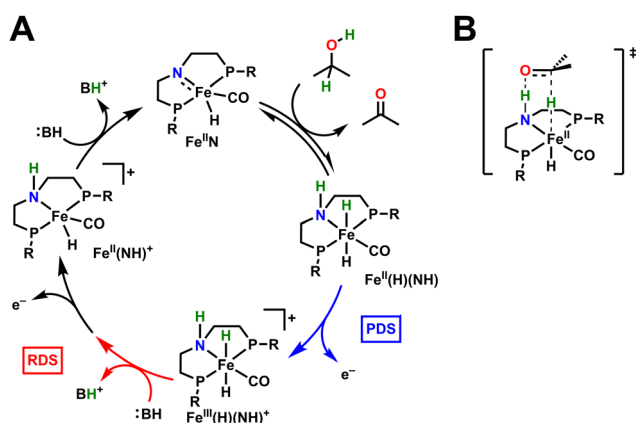
Fig. 4 (A) Catalytic cycle of Fe-pincer complex, FeN , proposed in McLoughlin et al. (R = i Pr 2 , :B = P 2 -Et). (B) Six-membered transition state involving a 2H + /2e − transfer between acetone to the metal center and PNP ligand.
