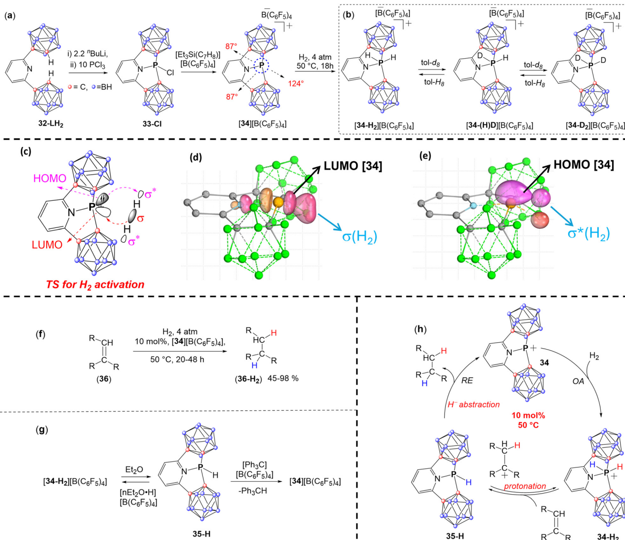
Fig. 13 Synthetic scheme for (a) the synthesis of [\mathbf{34}][\text{B(C}_6\text{F}_5)_4] ; (b) the activation of dihydrogen by [\mathbf{34}][\text{B(C}_6\text{F}_5)_4] and the exchange reaction between H and D atom between [\mathbf{34}\text{-H}_2][\text{B(C}_6\text{F}_5)_4] and toluene- \text{d}_8 and vice-versa; (c) schematic representation to show electrophilically driven activation of the H-H bond by \mathbf{34} ; (d) \sigma -bond of \text{H}_2 approaching the P-centre from the direction of the LUMO of \mathbf{34} ; (e) followed by the interaction of the HOMO of the P-centre with the LUMO ( \sigma^* ) of \text{H}_2 ; (f) [\mathbf{34}][\text{B(C}_6\text{F}_5)_4] catalyzed hydrogenation reactions of unsaturated C-C species; (g) equilibrium of [\mathbf{34}][\text{B(C}_6\text{F}_5)_4] with \mathbf{35}\text{-H} and reaction of \mathbf{35}\text{-H} with [\text{Ph}_3\text{C}][\text{B(C}_6\text{F}_5)_4] ; and (h) the proposed catalytic cycle.
