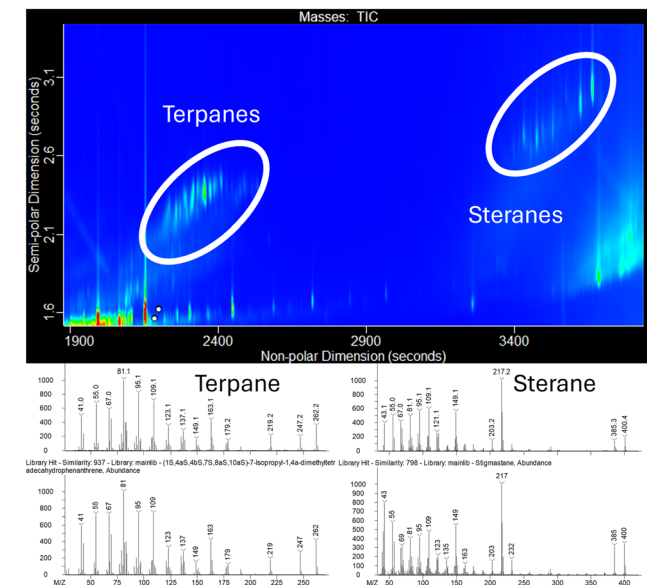
Fig. 9 GCxGC-MS contour plot (top) and one example of the EI mass spectra and library match spectra of one terpane and one sterane detected in undiluted HVO 4 (bottom).
