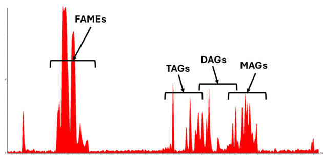
Fig. 10 Base peak ion current chromatogram (BPICC) of the positive ion ESI SFC-MS for HVO 6.
