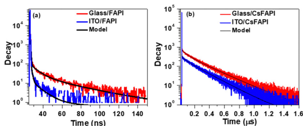
Fig. 6 Decay spectra of (a) FAPI, and (b) CsFAPI films. The black solid line is a fitting line from the bi-exponential decay function: I(t) = A + B_1e^{-t/\tau_1} + B_2e^{-t/\tau_2} + B_3e^{-t/\tau_3} .
