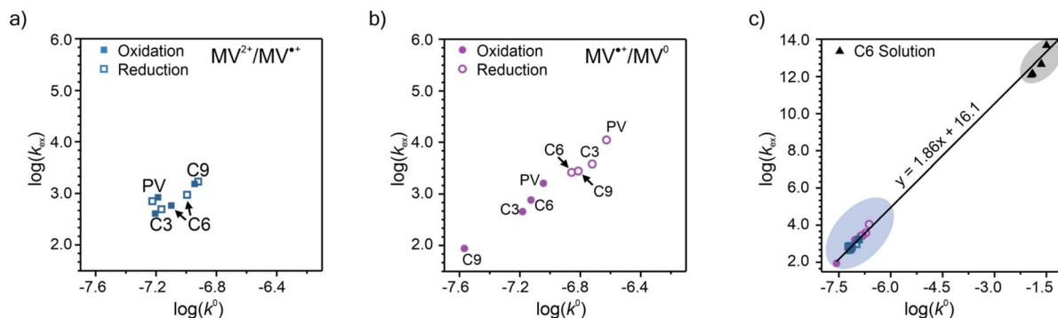
Fig. 5 Summary of the \log(k_{ex}) and \log(k^0) for PV, C3, C6, and C9. The results are presented as separate experimental values of oxidation and reduction for the (a) MV^{2+}/MV^{+•} and (b) MV^{+•}/MV^0 redox couples. (c) Plot showing all the \log(k_{ex}) vs. \log(k^0) for experimental data for both redox couples. Panels (a) and (b) show the enlarged region containing the CV/CA-determined rate constants for the viologen polypeptides studied in this work. In panel (c), the data points in the blue circle are from polymer thin-films and the data points in the black circle are from solution state values for a 0.2 mM solution of C6 dissolved in 0.5 M NaCl in H_2O (raw CA and CV data can be found in Fig. S33†).
