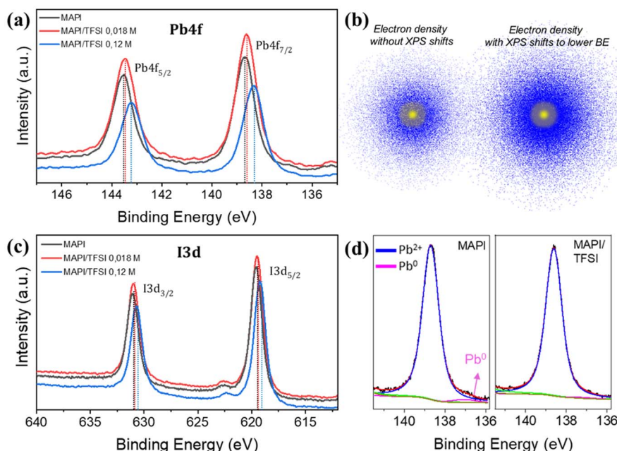
Fig. 3 Pb4f XPS spectra of MAPl and MAPl/TFSI films (a), schematic illustration of the correlation between XPS shifts and an atom's electron density (b), I3d XPS spectra (c) and Pb4f XPS spectra focused on 4f7/2 peaks (d) of MAPl and MAPl/TFSI films.
