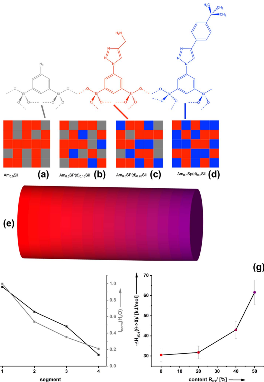
Fig. 6 (a–d) Schematic representation of the chemical nature of the pore-surfaces of Am_{x=0.5}Sp(d)_ySil materials which are constant in the amine density (red squares) and vary systematically in the spectator group (blue). For high y -values every amine has a spectator group as a neighbor and many have even two neighbors. (e) Schematic representation of a monolithic organosilica material containing a gradient in the spectator group R_{F2} = \textit{tert} -butyl phenyl. (f) Evaluation of FT-IR spectra of different segments associated with an increasing ratio of R_{F2} . (g) CO_2 adsorption enthalpies of materials associated with an increasing ratio of R_{F2} .
