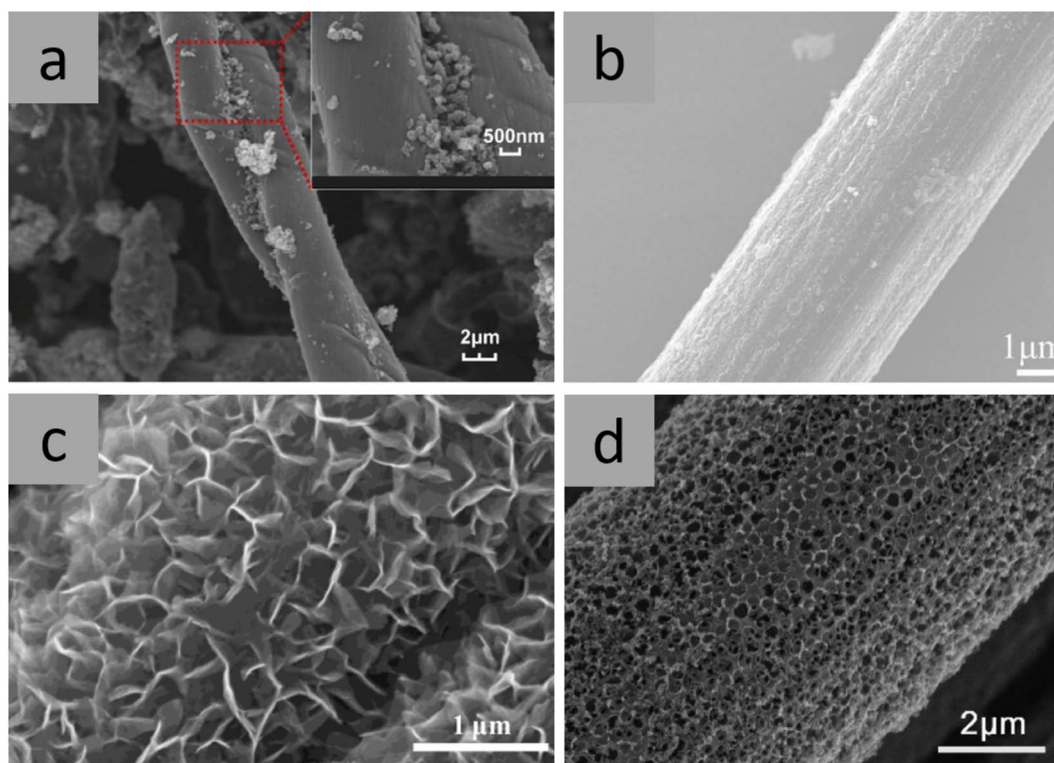
Fig. 6 Scanning electron microscopy (SEM) images of CFBA with different coating morphologies, including (a) inhomogeneous MnO, 45 (b) homogeneous Co 3 O 4 , 21 (c) V 2 O 5 nanosheets, 53 and (d) macroporous MoS 2 . 54 The void spaces in the MoS 2 coating were created by including polystyrene spheres in the coating that thermally decompose during annealing, demonstrating a creative use of the annealing process during the coating step. (a) Reproduced from ref. 45 with permission from Elsevier, copyright 2024. (b) Reproduced from ref. 21 with permission from Springer Nature, copyright 2024. (c) Reproduced from ref. 53 with permission from Elsevier, copyright 2024. (d) Reproduced from ref. 54 with permission from Wiley, copyright 2024.
