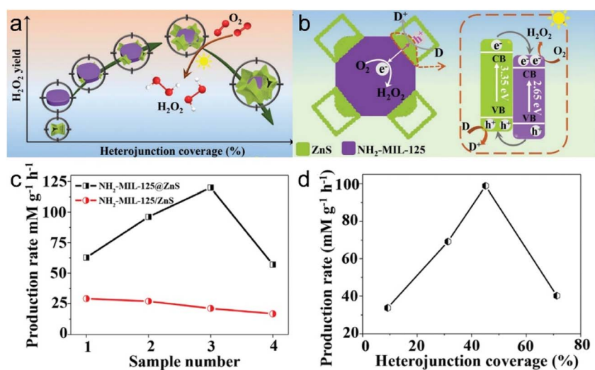
Fig. 15 (a) Diagram of (a) the relationship between H 2 O 2 yield and heterojunction coverage and (b) the band structure of NH 2 -MIL-125/ZnS heterojunction for photocatalytic O 2 reduction into H 2 O 2 . (c) H 2 O 2 production rate of NH 2 -MIL-125@ZnS and NH 2 -MIL-125/ZnS. (d) Normalized H 2 O 2 production rate. (Panels a-d) Reproduced with permission. 11 Copyright 2022, Wiley.
