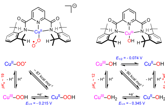
Scheme 6 Comparison of the thermodynamic properties of [(\text{L})\text{Cu}(\text{II})(\eta^1\text{-O}_2)]^- and [(\text{L})\text{Cu}(\text{III})(\text{OH})] using the same bis(arylcarboxamido)-pyridine ligand. Adapted from ref. 103.
