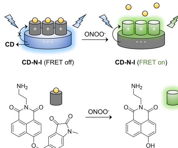
Scheme 1 Schematic diagram of the mechanism of peroxynitrite detection using CD-N-I.
