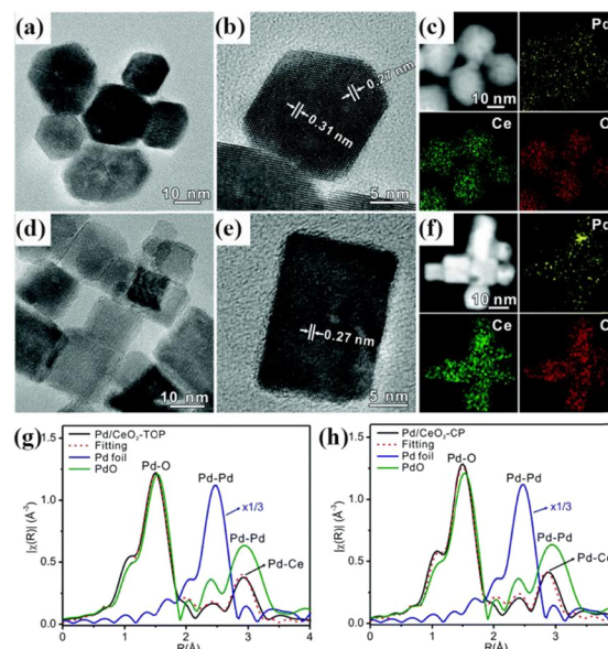
Fig. 7 (a) and (d) TEM and (b) and (e) HRTEM images of \text{Pd}/\text{CeO}_2 -TOP and \text{Pd}/\text{CeO}_2 -CP prepared via a photochemical route. (c) and (f) HAADF-STEM images of \text{Pd}/\text{CeO}_2 -TOP and \text{Pd}/\text{CeO}_2 -CP, and their corresponding EDX mappings of Pd, Ce, and O; Fourier transforms of EXAFS spectra for (g) \text{Pd}/\text{CeO}_2 -TOP and (h) \text{Pd}/\text{CeO}_2 -CP as well as the reference materials Pd foil and PdO at the Pd K-edge. Reproduced with permission. 33 Copyright 2017, The Royal Society of Chemistry.
