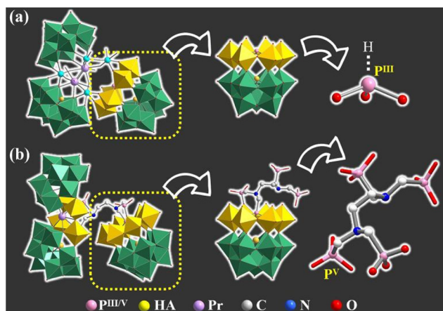
Fig. 3 Comparison of the inorganic HP III -inserted Dawson-like (HP III SeW 15 ) unit in 2a (a) and the organic-inorganic hybrid {C 6 N 2 P 4 SbW 15 } unit in 1a (b).
