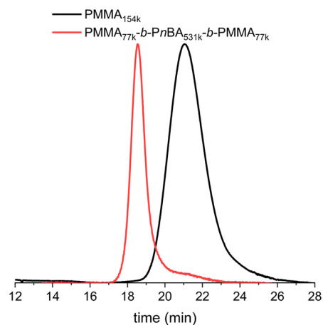
Fig. 4 SEC-RI chromatograms of \text{PMMA}_{154k} and the corresponding \text{PMMA}_{77k}\text{-}b\text{-}Pn\text{BA}_{531k}\text{-}b\text{-}PMMA_{77k} triblock copolymer.
