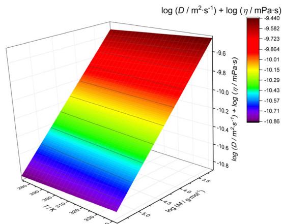
Fig. 3 3D calibration fit of viscosity-corrected diffusion coefficients (obtained using dstebppg3s ) as a function of temperature and the molar mass of polystyrene standards.
