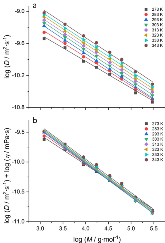
Fig. 2 (a) Diffusion coefficients determined via DOSY for polystyrene standards at several temperatures measured using the better dstebppg3s pulse sequence and (b) viscosity-corrected calibration data for the same measurements.
