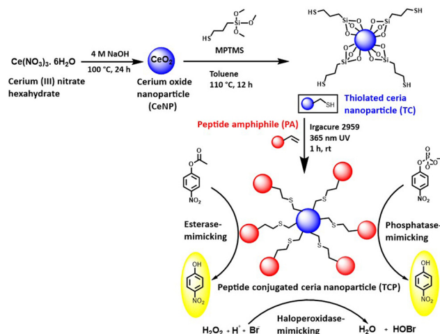
Scheme 1 Fabrication of thiol-functionalized ceria nanoparticles and their conjugation to branched peptide amphiphile via thiol-ene conjugation for esterase, phosphatase, and haloperoxidase-mimicking activities.
