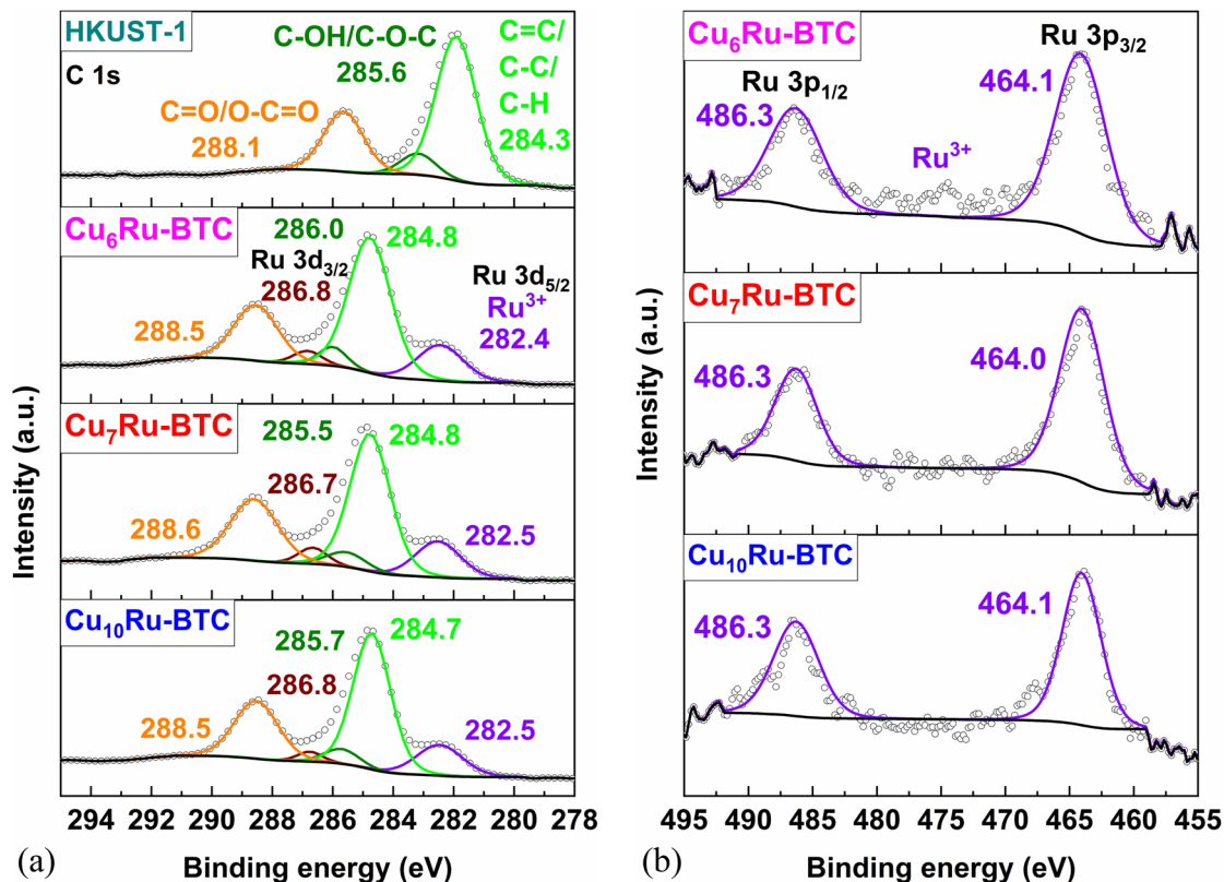
Fig. 5 HR-XPS spectra of (a) C 1s and Ru 3d and (b) Ru 3p for \text{Cu}_{10}\text{Ru-BTC} , \text{Cu}_7\text{Ru-BTC} , \text{Cu}_6\text{Ru-BTC} and mechanochemically synthesized HKUST-1.
