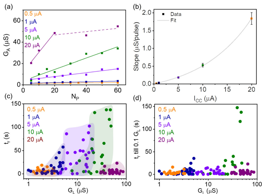
Fig. 5 Building up of the G profile. (a) Variation of G_A with N_p for different I_{CC} . (b) Slopes from the linear fits in (a) as a function of I_{CC} . For 20 \mu A I_{CC} the slope refers to the first three data points before G saturates. G_L and t_r relation. (c) Variations in t_r with G_L for different I_{CC} . Free-form shapes enclose the individual sets of data where the data spread is due to varied N_p (5 to 60). (d) t_r of G till 0.1G_L (i.e., 90% drop of G_L ) as a function of G_L . ( V_p \sim 2 V, V_R \sim 30 mV) ( t_w and t_i \sim 50 ms).
